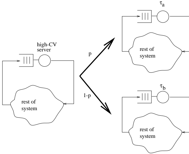
Figure 2: System Decomposition
