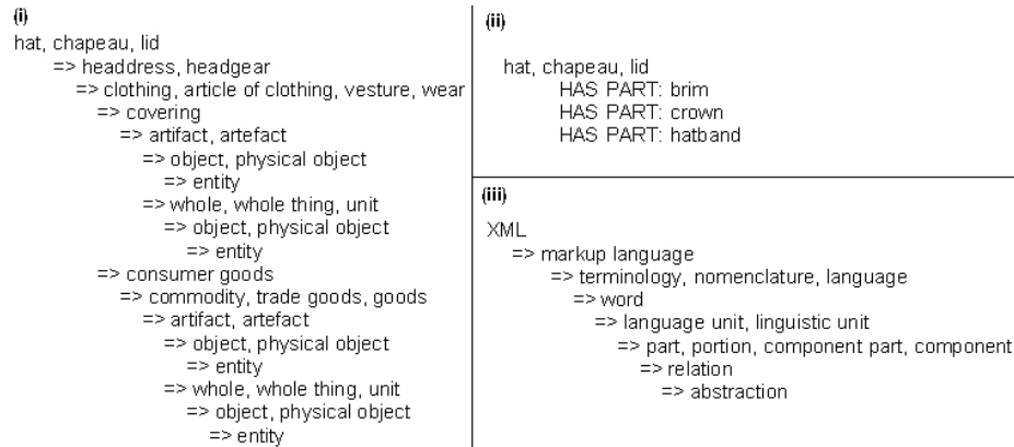
Fig. 1. Examples from the WordNet lattice: (i) shows the lattice for the first sense of “hat”. (ii) shows the meronyms or parts of a hat. (iii) shows how we can add a term “XML” to extend the WordNet lattice with new terms.
