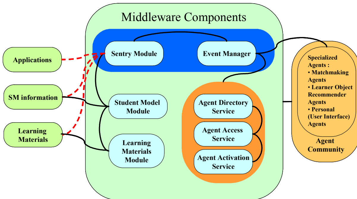
Figure 1: Middleware components
