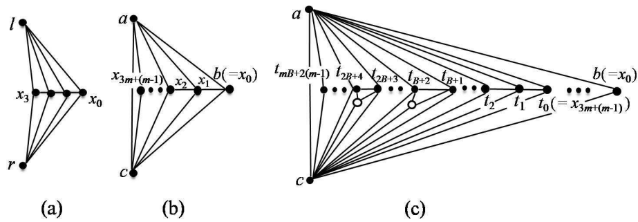
Fig. 3. (a) W_4 , (b) W_{4m} , together with an edge (a, c) between the wings a and c , and (c) illustration for G' , where the buds are shown by empty circles.
