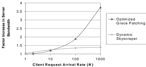
Figure 5: Previous Techniques Relative to Early Merging
