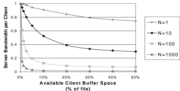
Figure 4: Bandwidth Requirements of Early Merging
