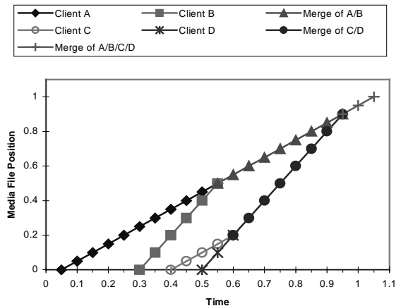
Figure 2: Example Merge Tree
