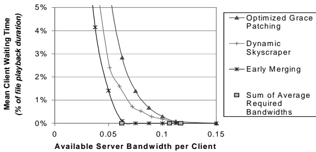
Figure 6: Mean Client Waiting Times
