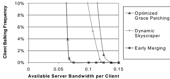
Figure 7: Client Balking Frequencies
