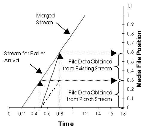
Figure 1: Stream Merge Operation
