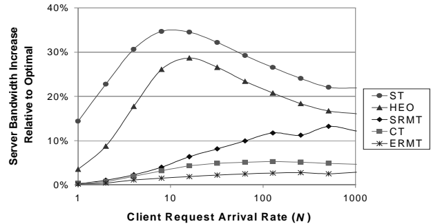
Figure 3: Performance Relative to Optimal Stream Merging
