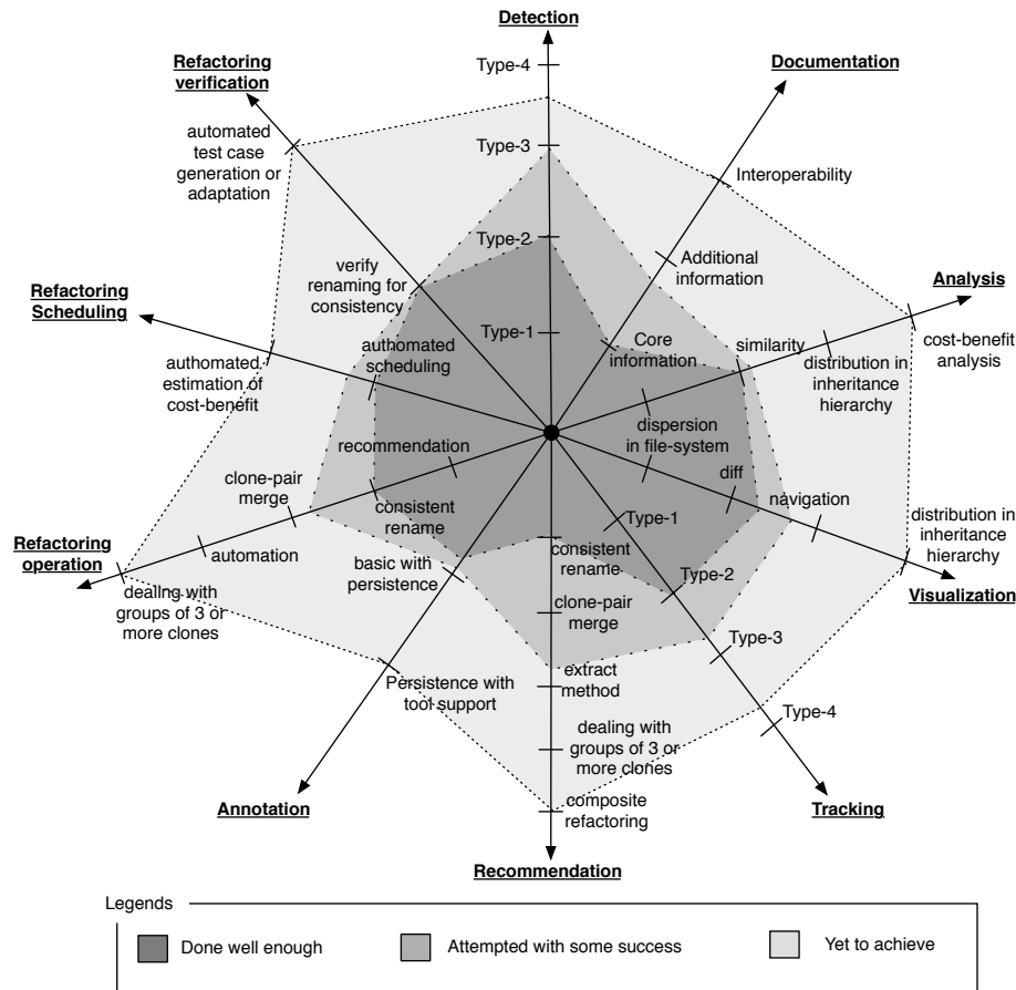
Fig. 5. Achievements and scopes along different dimensions of clone management activities
